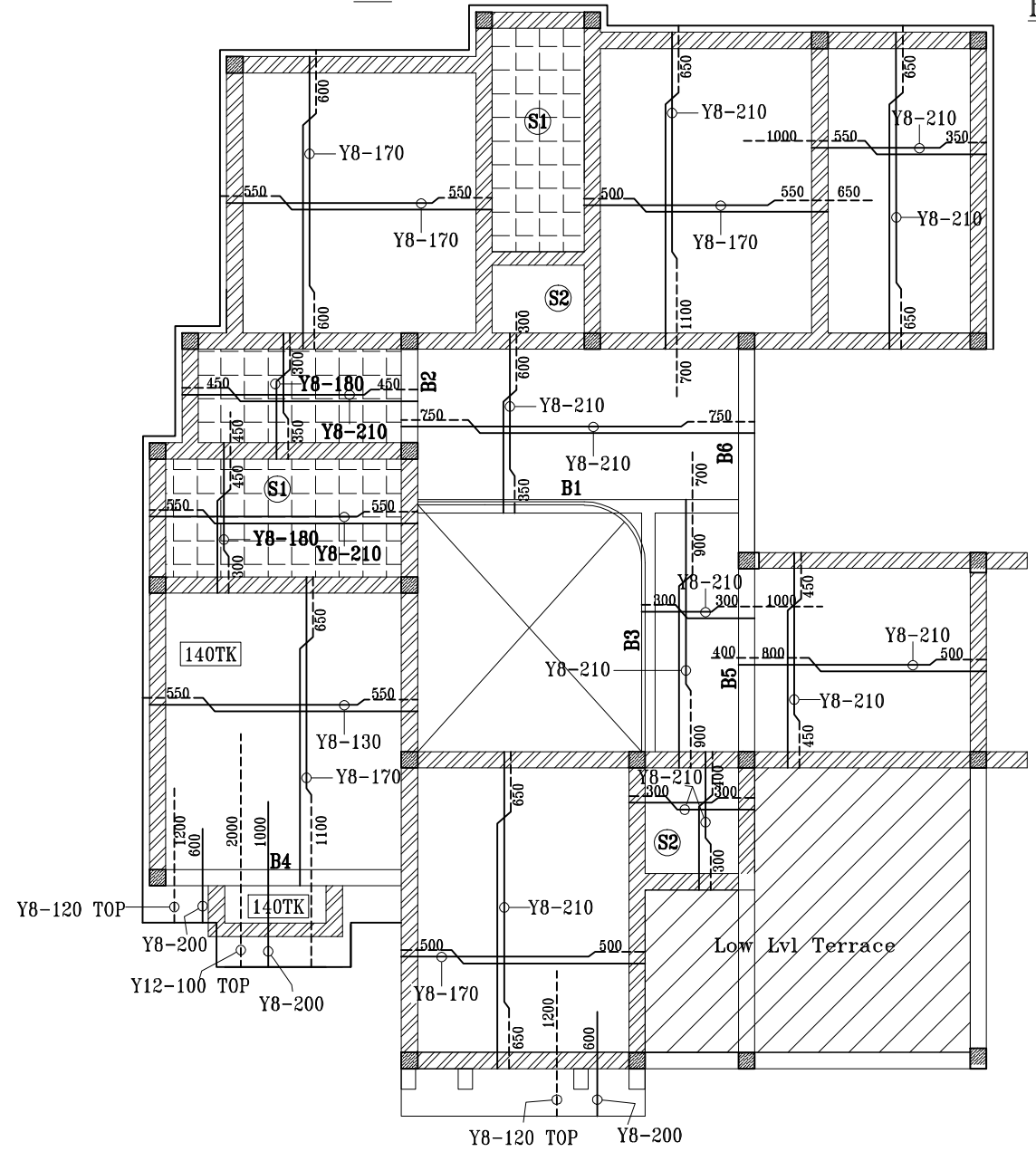
FIRST FLOOR DETAILS
